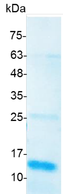
SDS-PAGE analysis of recombinant human BMP-3
